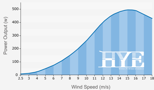
HY- 400 Wind Turbine Power Curve
