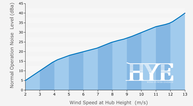
Wind Turbine Noise Level on HY-1500 (Standard Air Density(1.225 kg/m 3 ))
